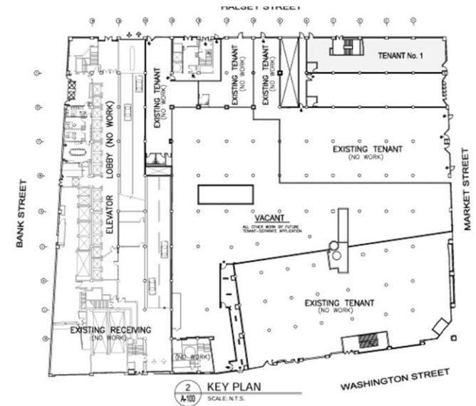
LEASE PLAN JJ OPERATING INC. 131 MARKET STREET, NEWARK, NEW JERSEY
